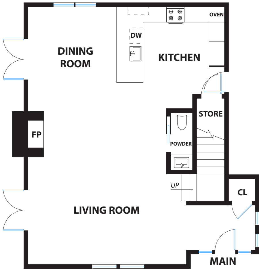
FIRST FLOOR
