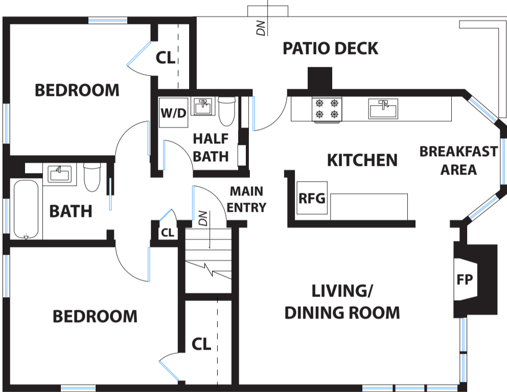
MAIN LEVEL
