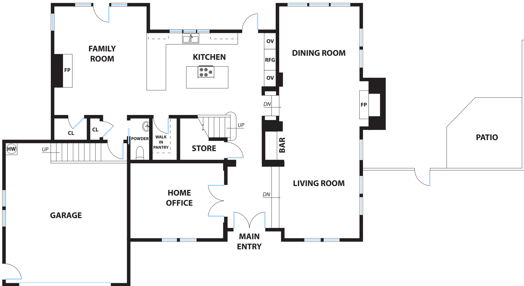
FIRST FLOOR
