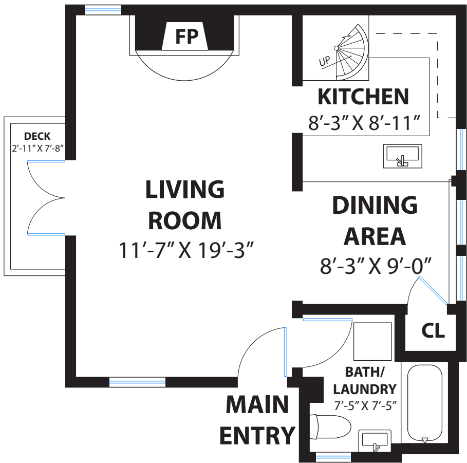
MAIN LEVEL
