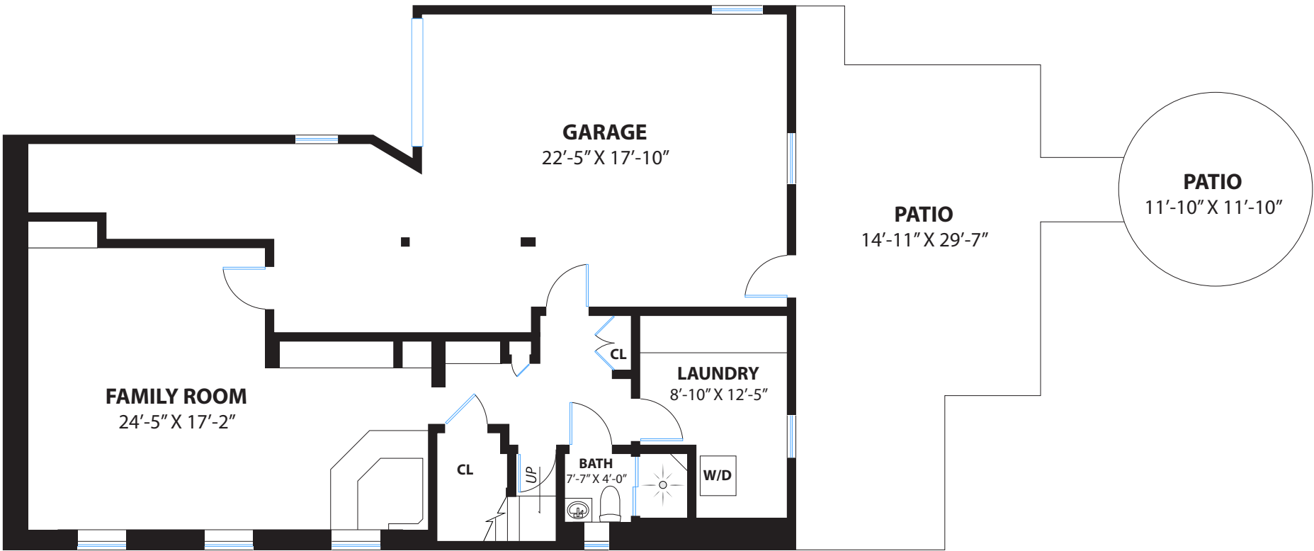
LOWER FLOOR
