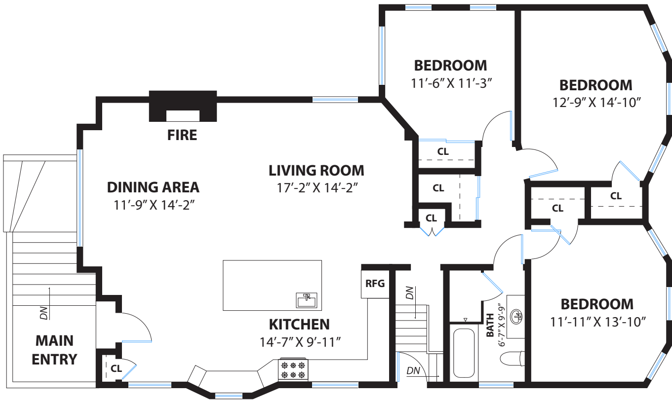
MAIN FLOOR
