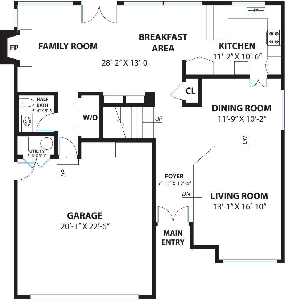
MAIN LEVEL
