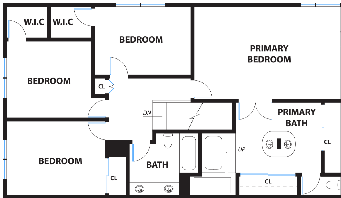
SECOND FLOOR
