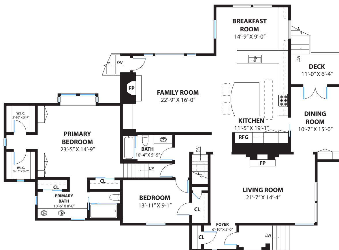
MAIN LEVEL
