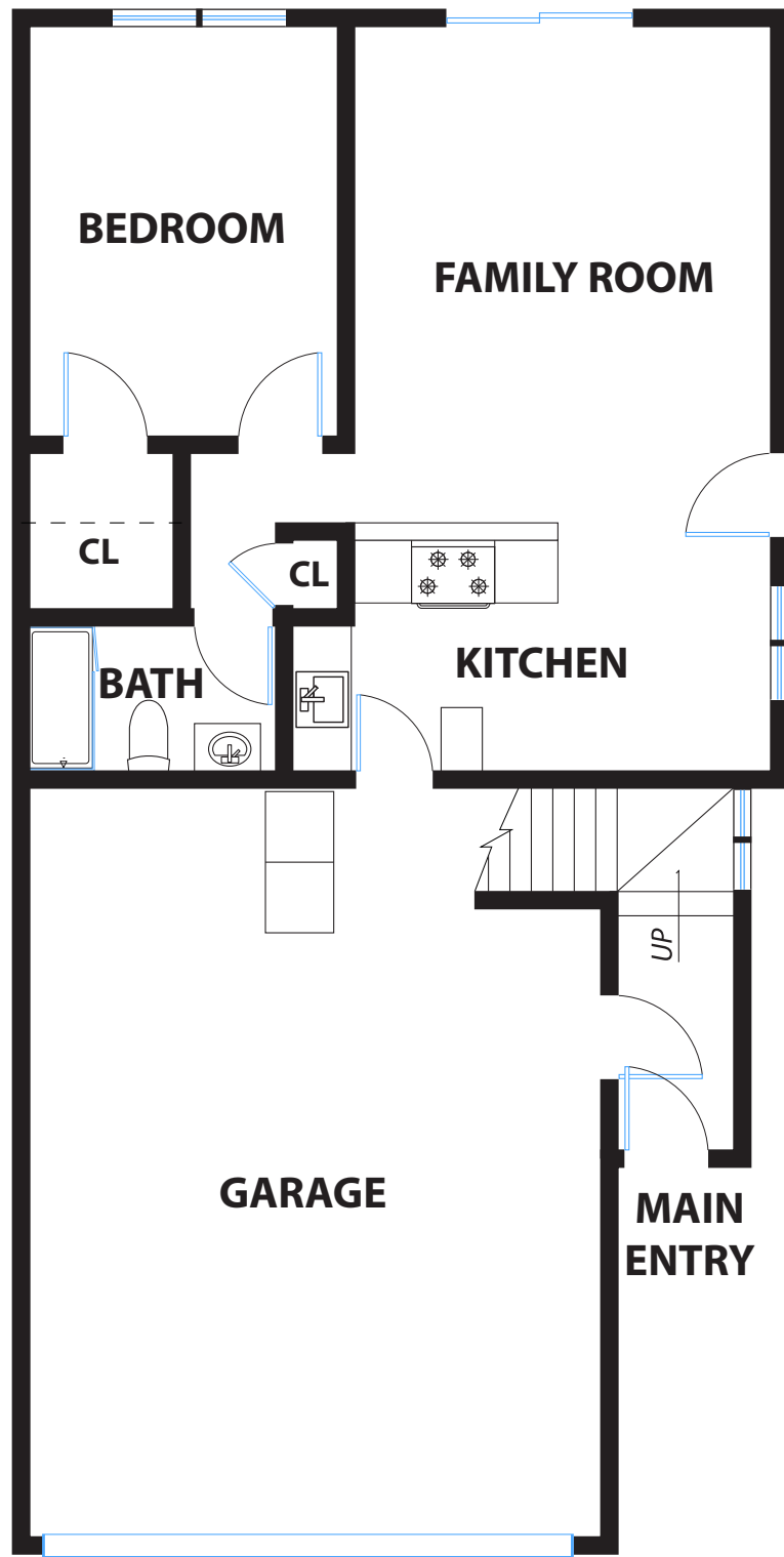
GROUND FLOOR
