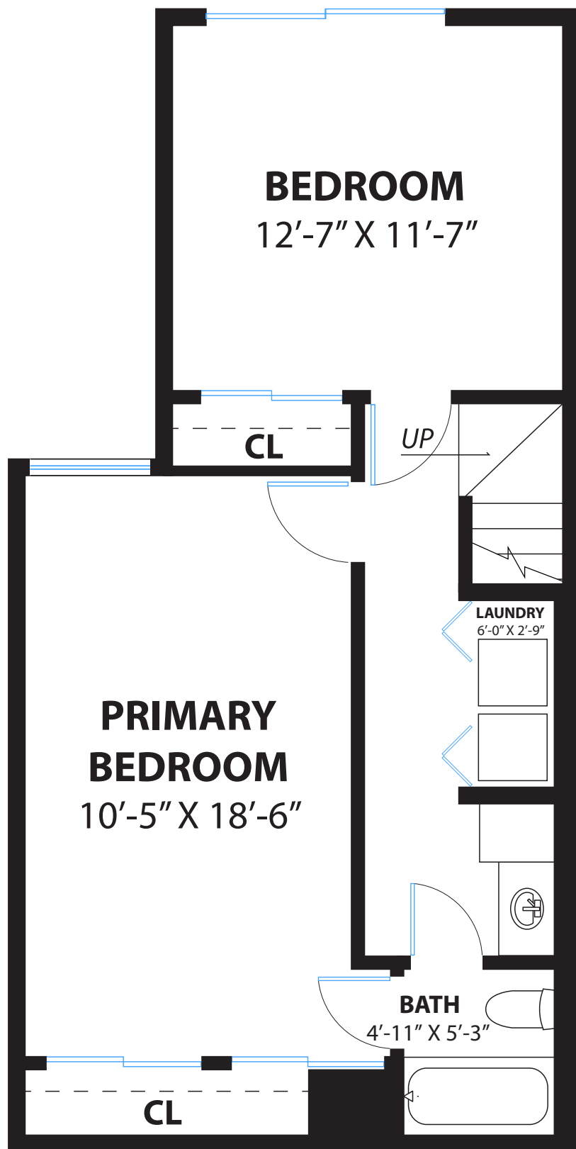
FIRST FLOOR
