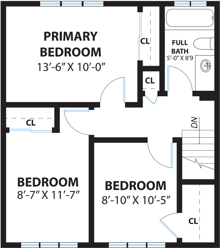
UPPER FLOOR
