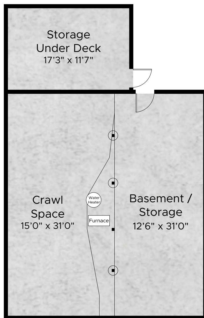
Basement Level
