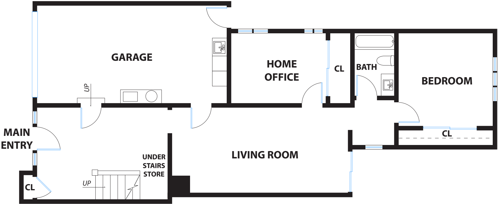
FIRST FLOOR
