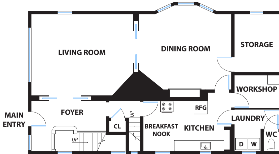
SECOND FLOOR
