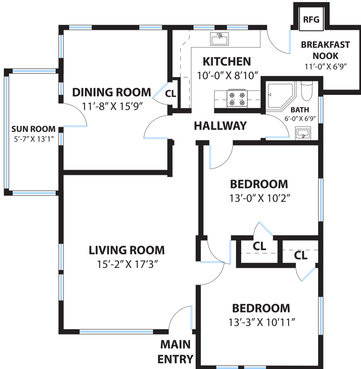
SECOND FLOOR
