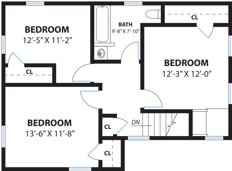
UPPER LEVEL
