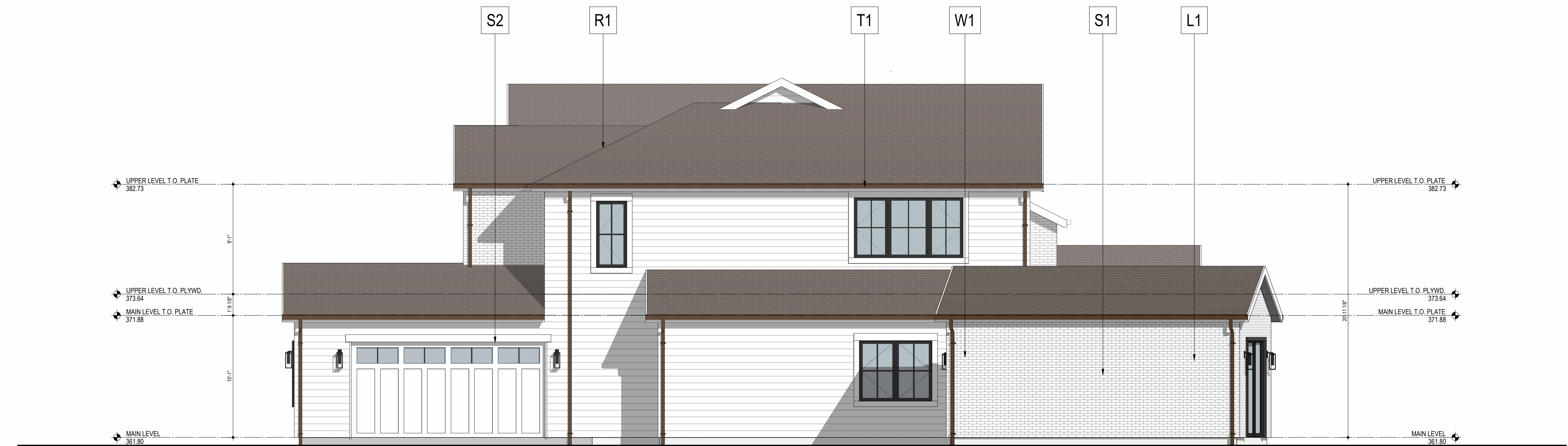
2 NORTH ELEVATION 00 02 04 08 FEET 1/4" = 1'-0"
