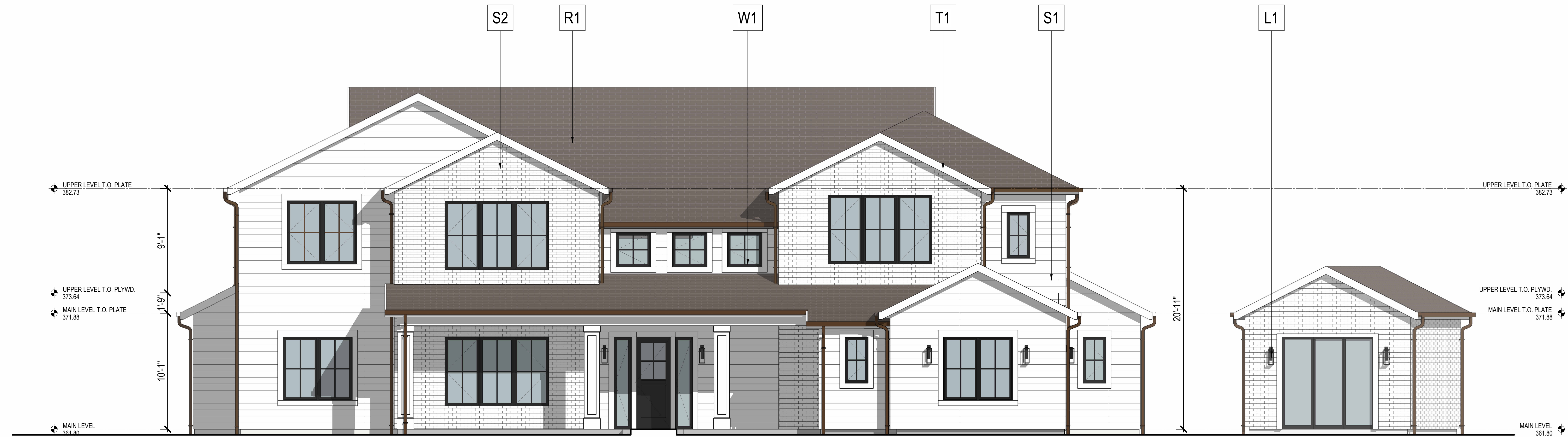
1 EAST ELEVATION 00 02 04 08 FEET 1/4" = 1'-0"
