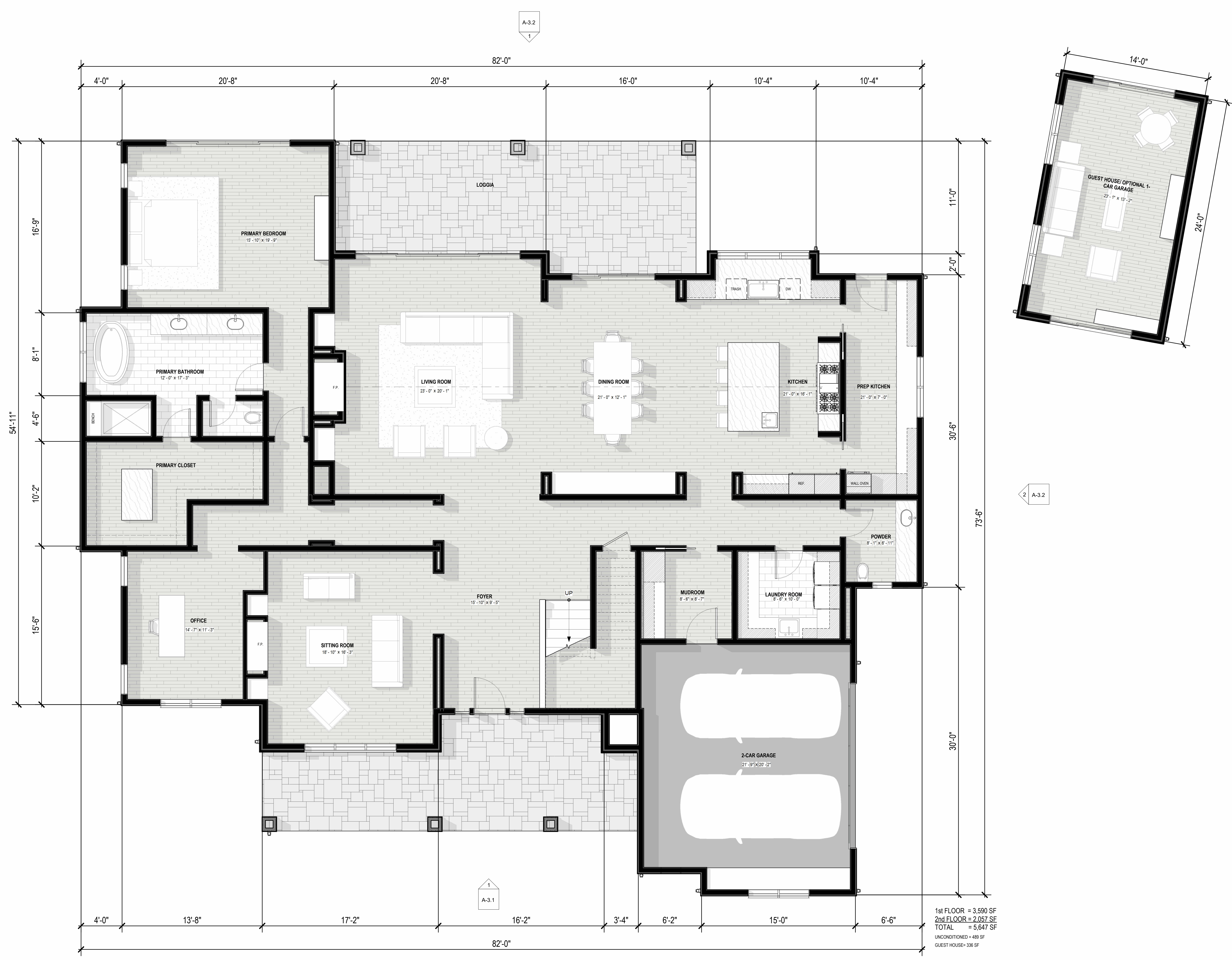
1 FIRST LEVEL FLOOR PLAN 00 02 04 08 FEET 1/4" = 1'-0" S N
